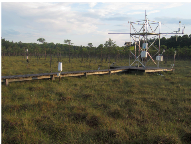
Eddy covariance measurements of GHG (Kusowo Bog, Poland).
